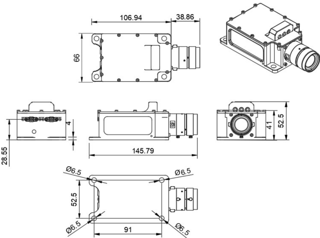
FIGURE 1 MECHANICAL DRAWING OF RLT-NG1-001 CAMERA
