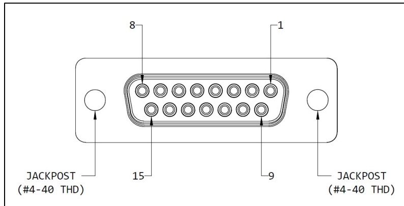
Figure 5. SND15S36000G Connector Mating Face View
