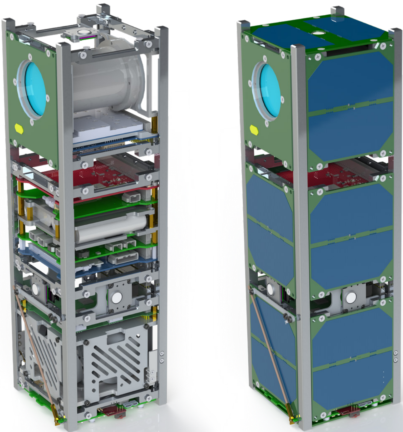
Picture 2 – SXC3 layout
