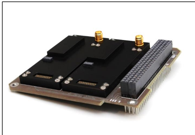
Two radios stacked on the same PCB/104
